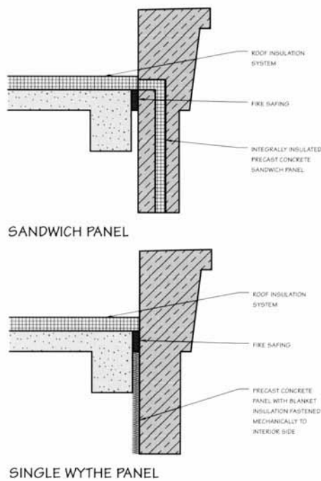
Figure 1 Wall insulation can mate easily with roof components, providing a tight seal, whether an insulated sandwich wall panel (top) or a single concrete wythe (bottom) is used.
