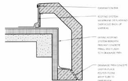
Figure 3 To prevent leakage, Fend adds an extra piece of conventional base flashing over the back of panels along the roofline, flashed out at the extended roof membrane beneath the C-shape.
