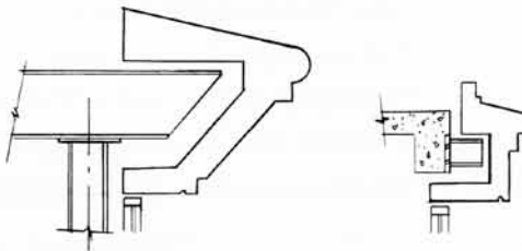
Figures 3-7B & 3-7C Special Structural Supports
