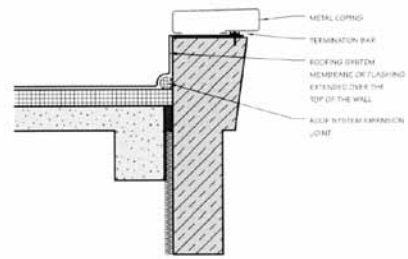
Figure 2 With a straight-backed cornice panel, Fend completes the roof detail with a metal, stone or precast coping piece to hide the termination.
