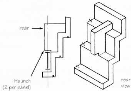
Figure 3-7A Special Haunch on Panel
